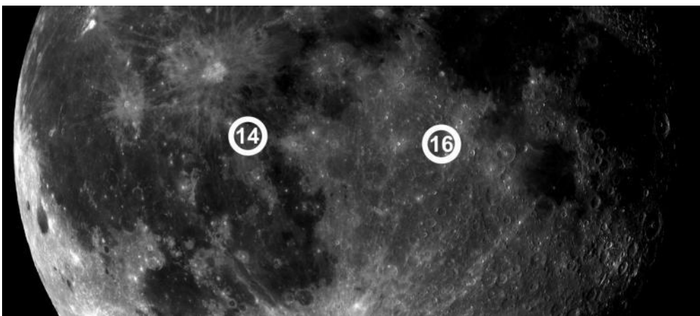
Figure 1: Landing sites of the Apollo 14 and 16 missions
