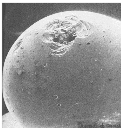
Figure 2: Micro-crater (0.3mm) on a glass particle from the Lunar surface Contact
